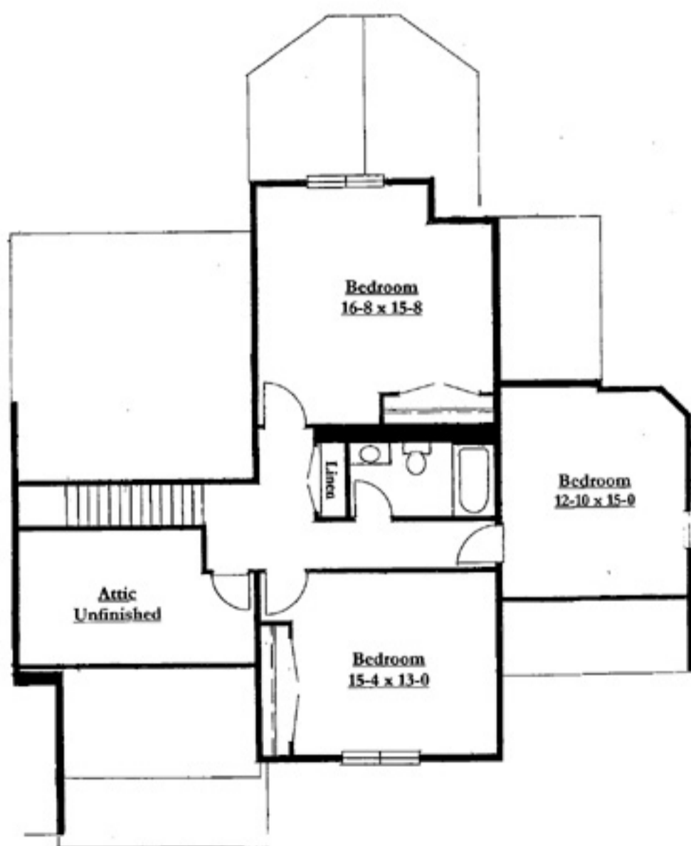
Ten Fellows Lane Second Floor Plan
