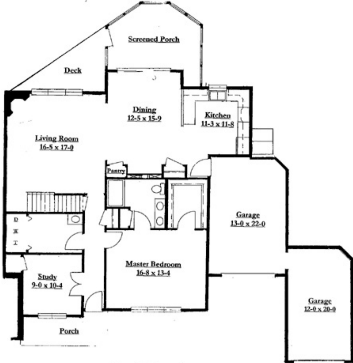
Ten Fellows Lane First Floor Plan
